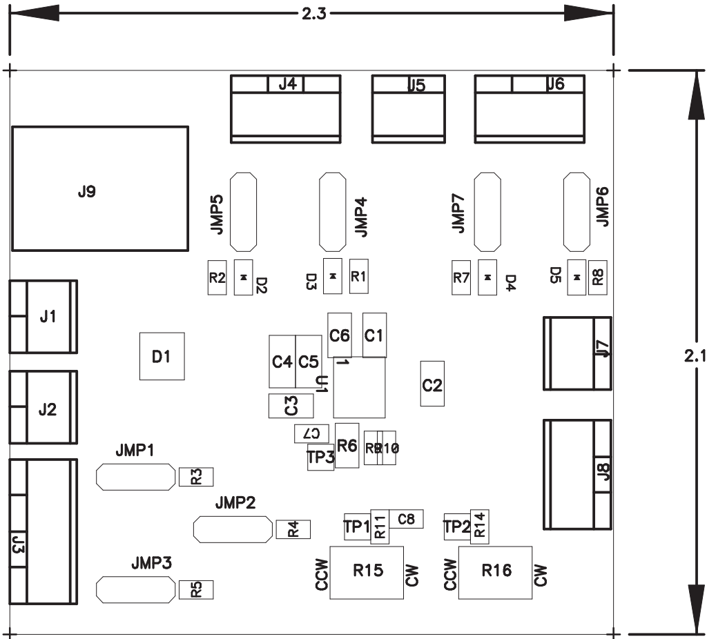
Figure 3. Top Assembly View
